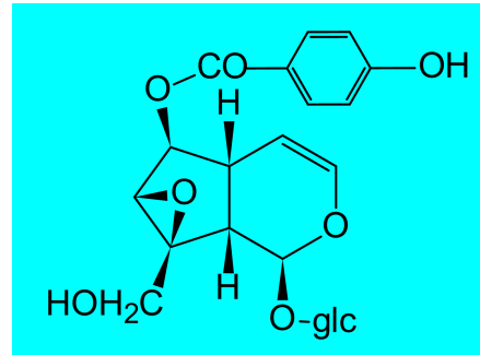
梓苷
